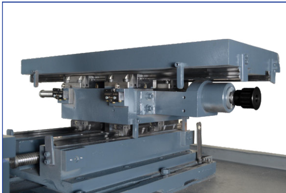
Pic: Linear Motion Guideways and C3 class ballscrews
